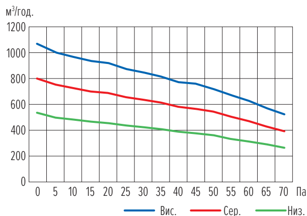
MCFDS-085-AT2
