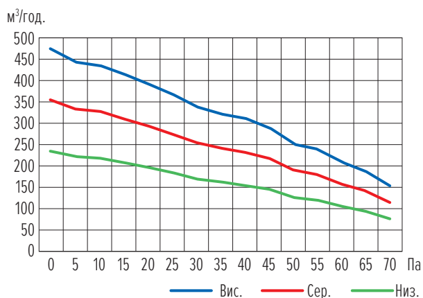
MCFDS-034-AT2
