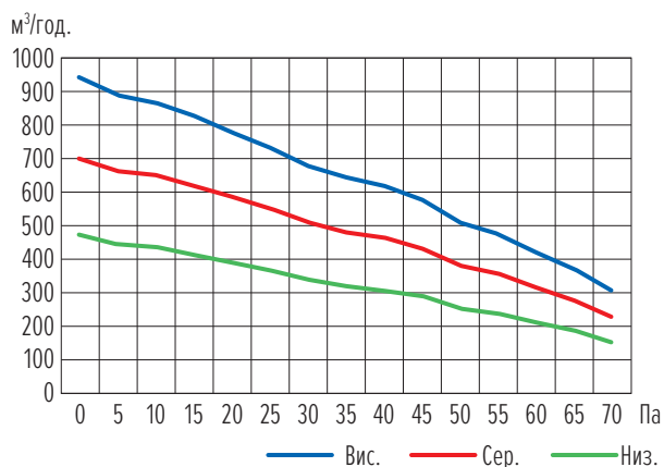
MCFDS-068-AT2
